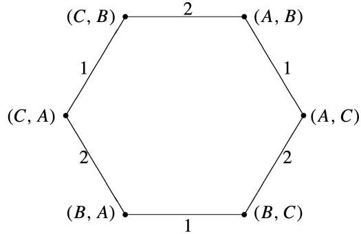
Figure 1: Frame describing a simple card game
