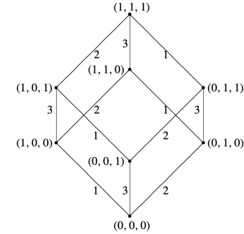
Figure 2: Frame for the muddy children puzzle with n = 3
